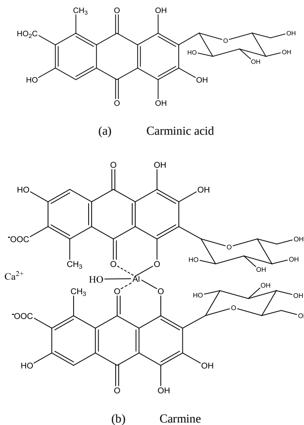
Figure 1: Structural formulae, according to Harris (2009), for (a) carminic acid and (b) carmine
